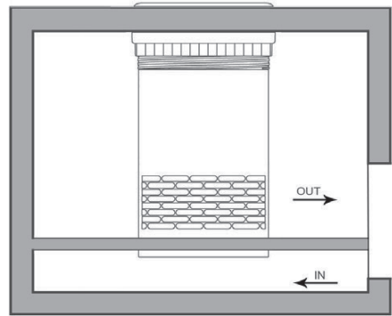
Unique venting grid
