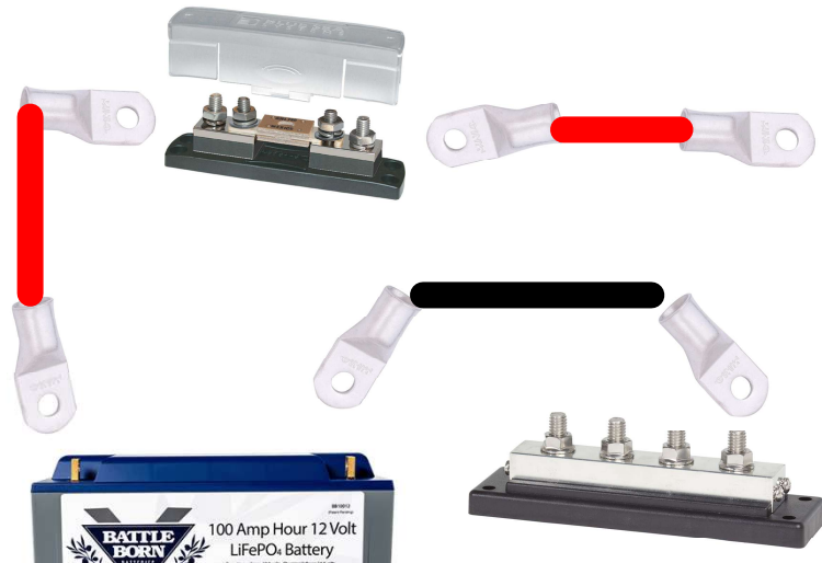
Supplied DC Positive wiring harness
